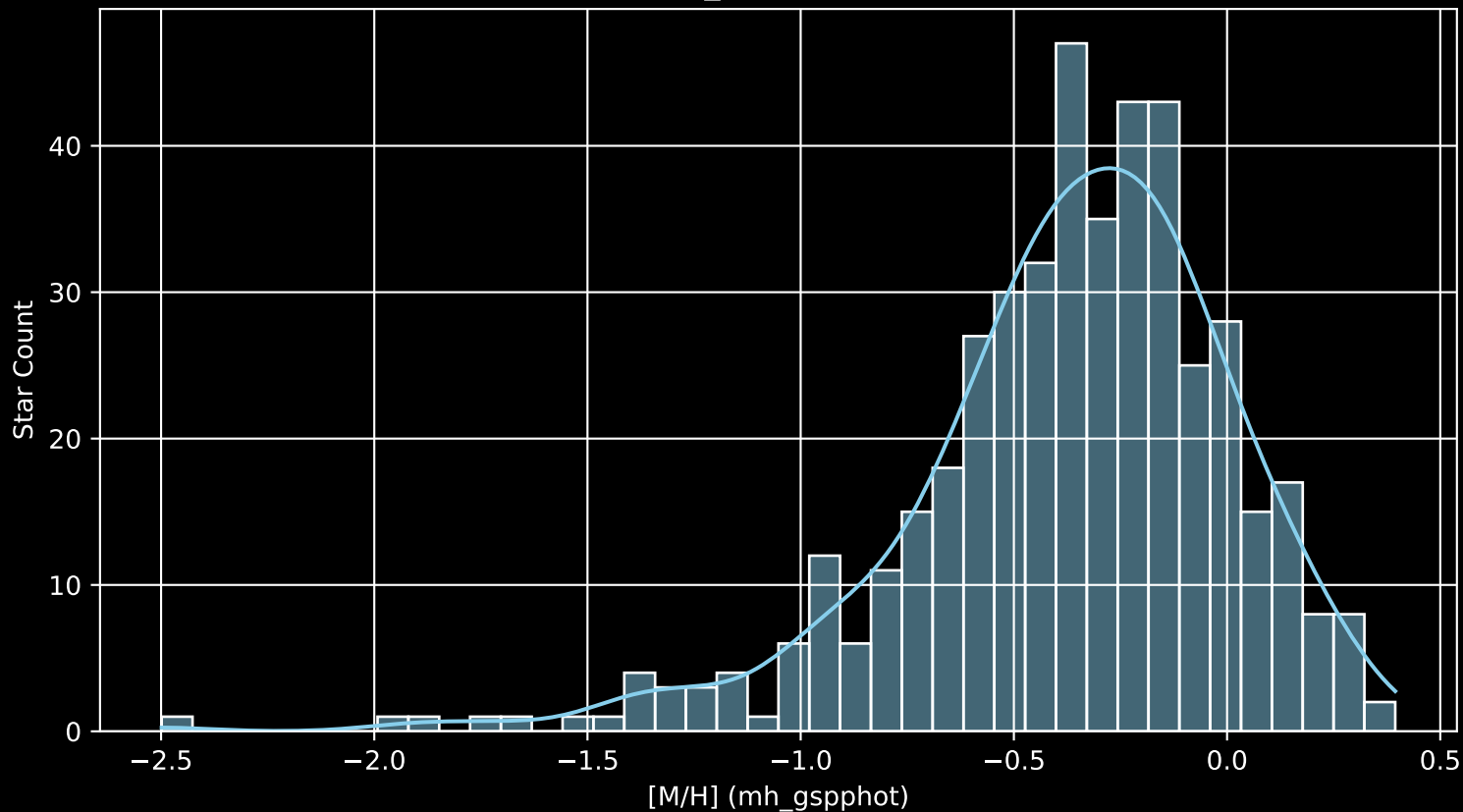
APOGEE DR17 Field: [M35N2158_btx [M/H] (mh_gspphot) (n= 450)
