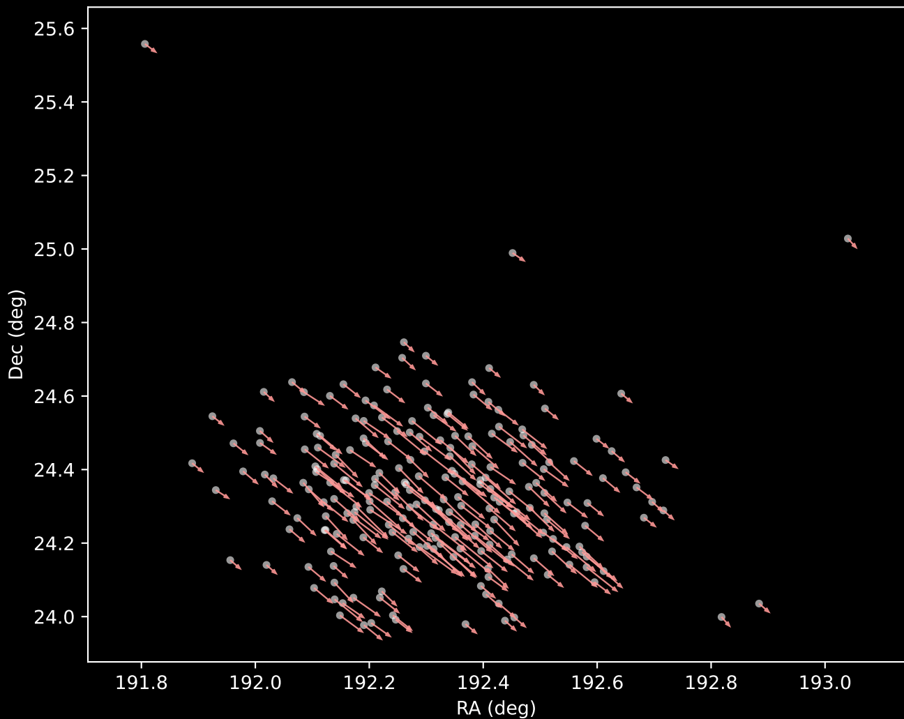
APOGEE DR17 Cluster 7 Proper Motion Vectors (n=218)
