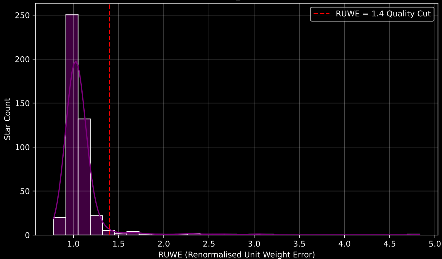
GAPOGEE DR17 Field [M35N2158_btx] RUWE Distribution (n= 447)
