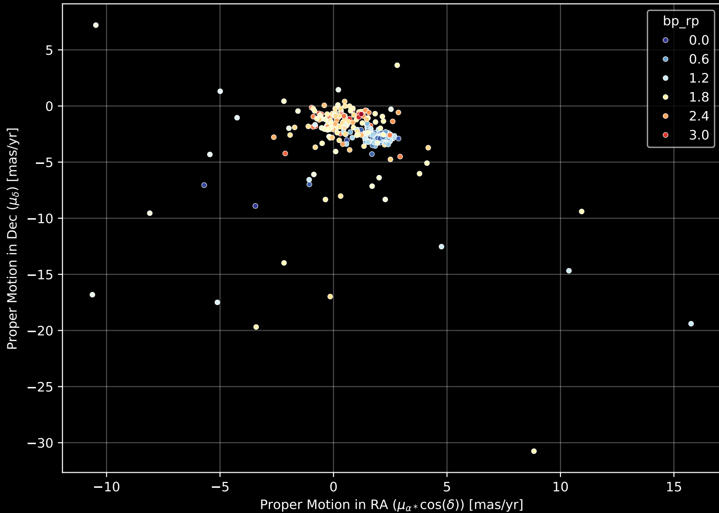
APOGEE DR17 Field: [M35N2158_btx] Proper Motion Diagram (n= 453)
