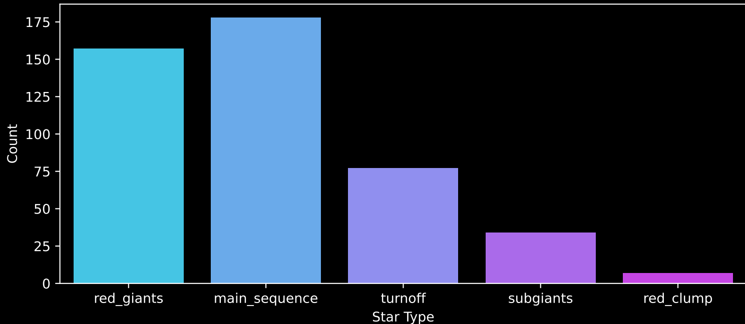
APOGEE DR17 Field: [M35N2158_btx] Count plot of Star Type
