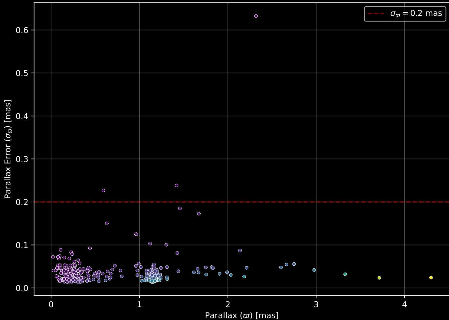
APOGEE DR17 Field: [M35N2158_btx] Parallax Quality (n= 453)
